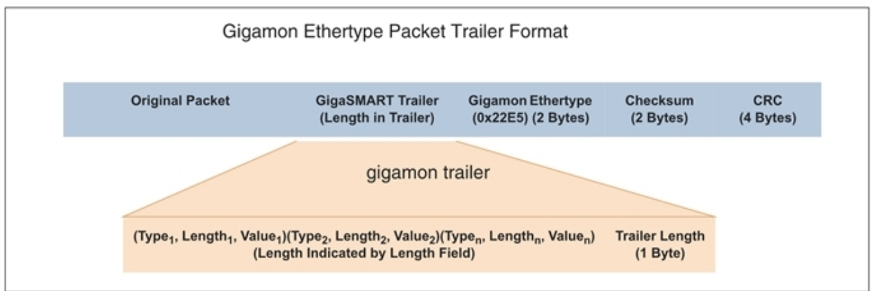
Figure 173 GigaSMART Trailer Format
