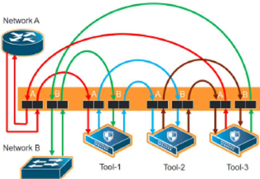
Figure 109 Inline Tool Series Per-Direction: Forward
