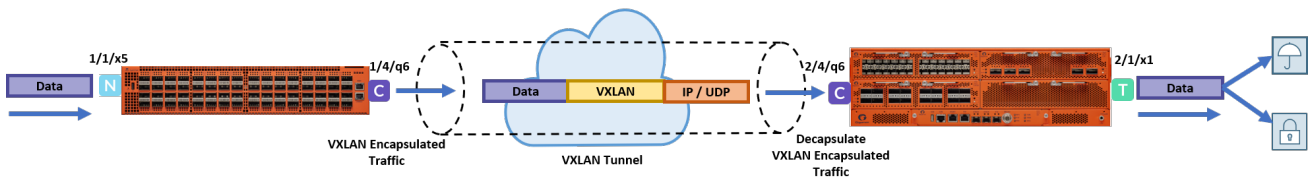
Figure 32 VXLAN Tunnel Encapsulation and Decapsulation
