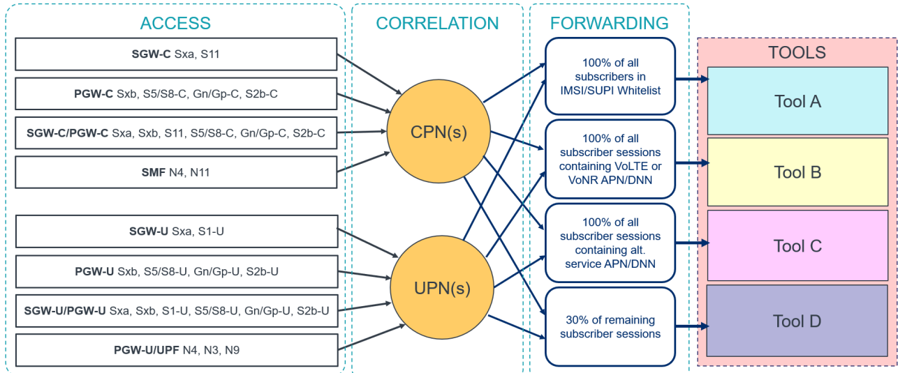
Figure 33 CUPS Traffic Visibility Solution
