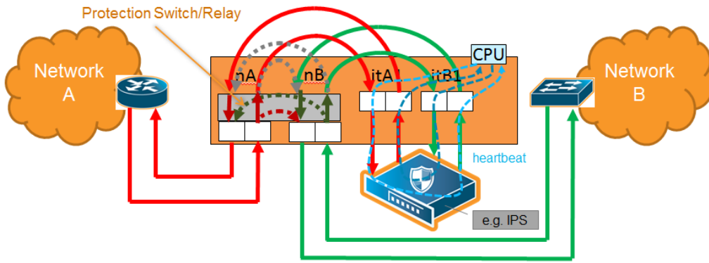
Figure 75 Simple Configuration
