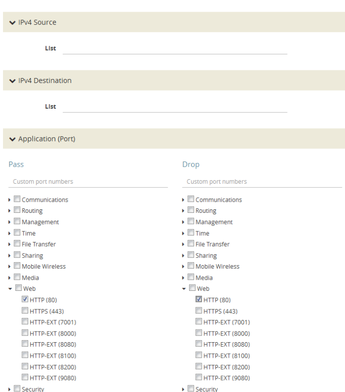
Figure 46 Custom Port Number Selected in Quick Rule Editor
