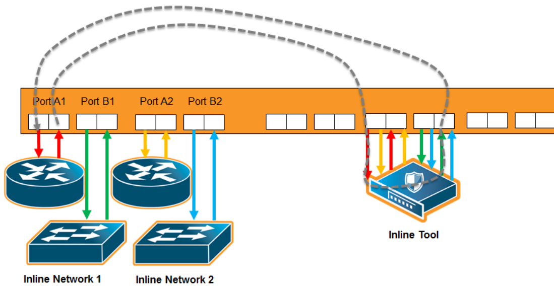
Figure 78 Inline Network Group
