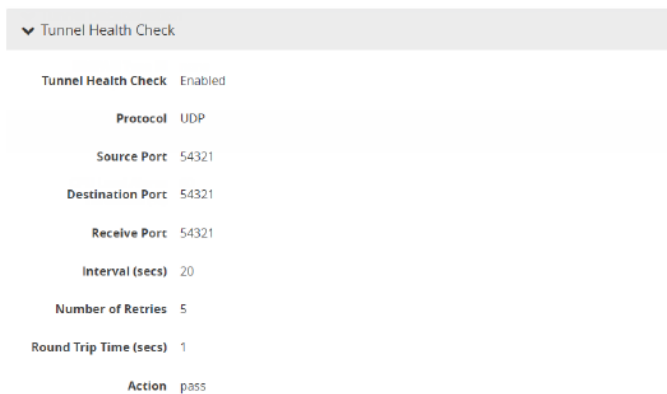
Figure 157 Configure UDP Health Check Parameters
