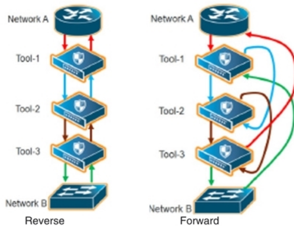
Figure 107 Inline Tool Series Per-Direction Order: Simplified Reverse and Forward
