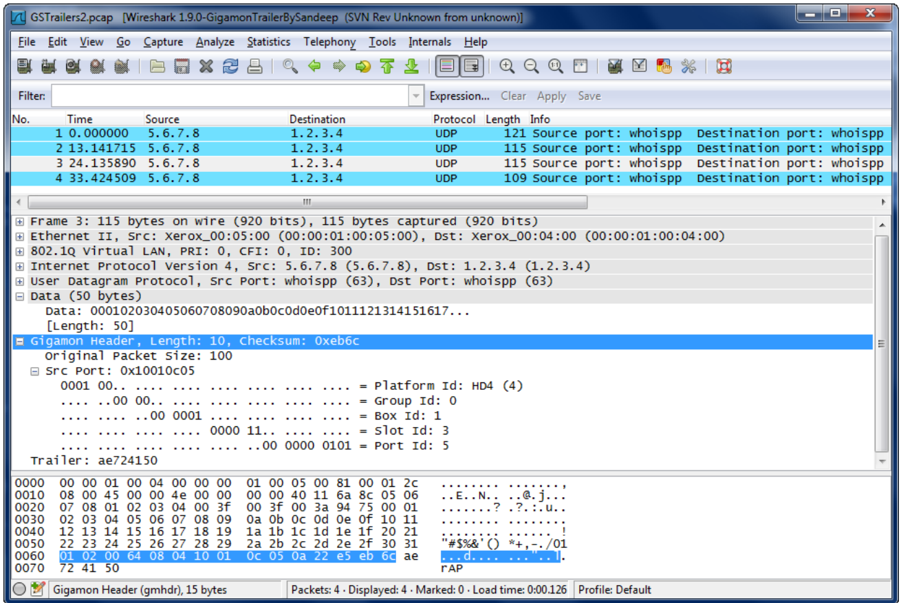
Figure 174 Wireshark Decode of GigaSMART Trailer
