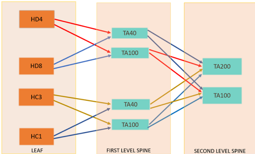
Figure 66 Spine to Spine and Leaf cluster overview,
