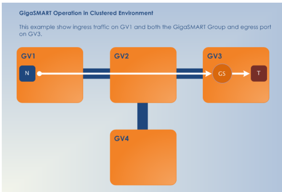
Figure 163 GigaSMART Operations in Clusters
