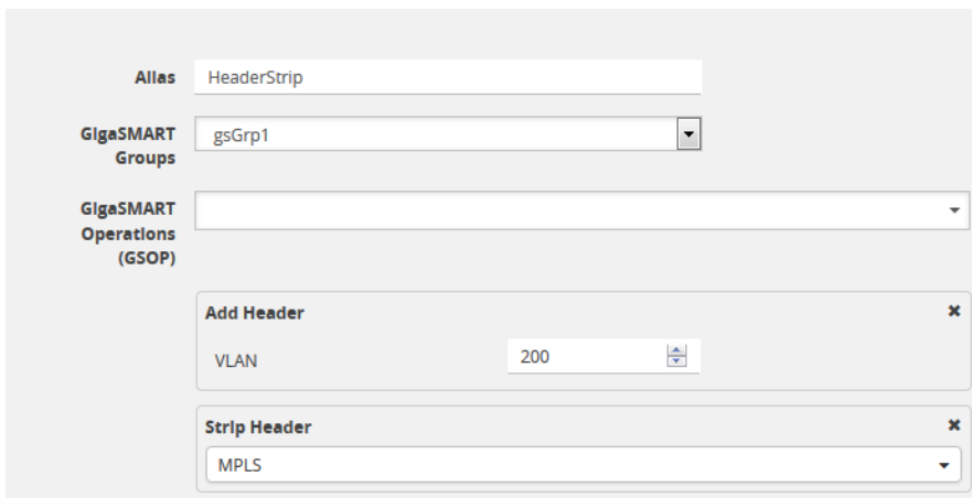
Figure 56 Strip Header GigaSMART Operation for Stripping MPLS Headers
