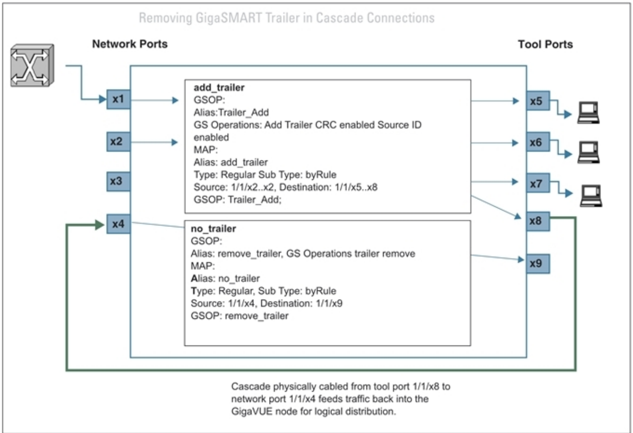
Figure 172 Removing the GigaSMART Trailer from a Cascade Connection
