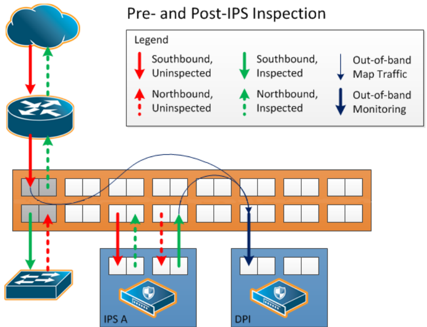
Figure 80 Out-of-Band Arrangement
