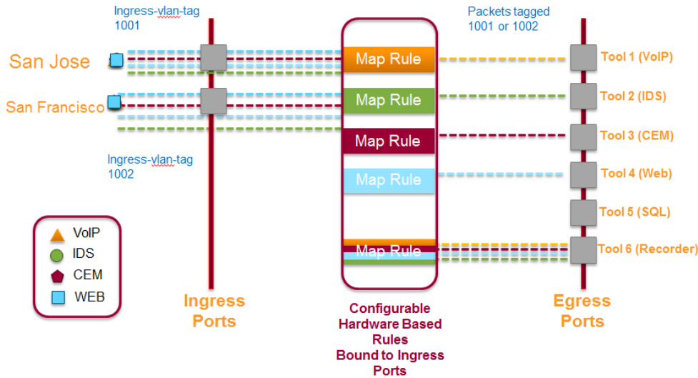
Figure 13 Using Ingress Port VLAN Tagging
