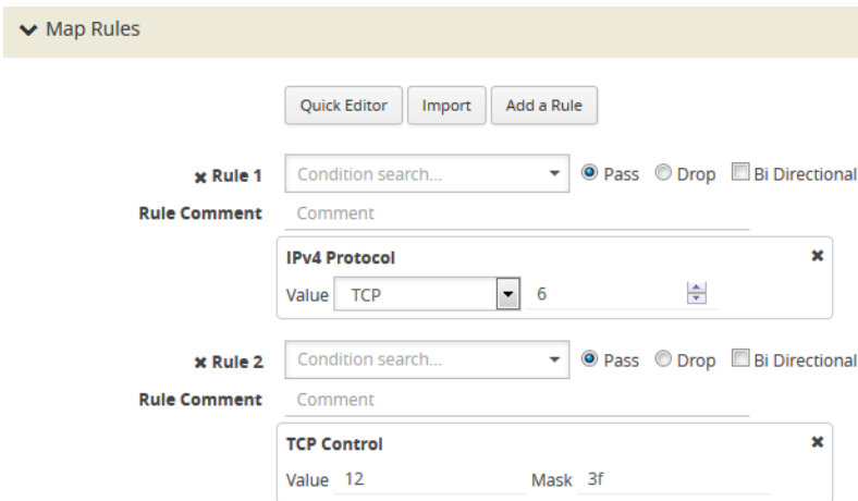
Figure 37 Map Rule Matching All Packets with Both ACK and SYN Bits set
