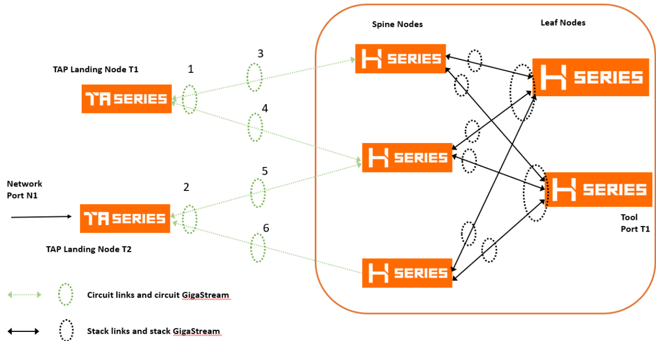
Figure 133 Leaf-Spine Based Topology.
