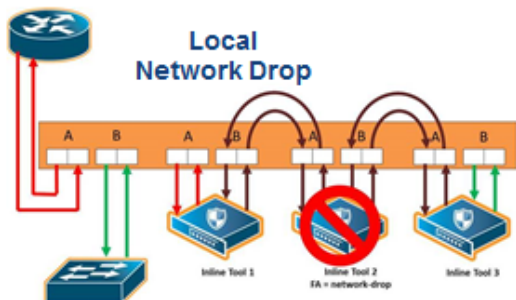
Figure 104 Inline Tool Series Local Network Drop Failover Action
