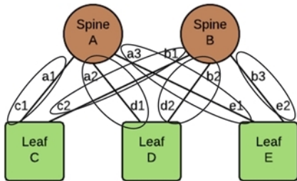
Figure 37 Stack Link Configuration
