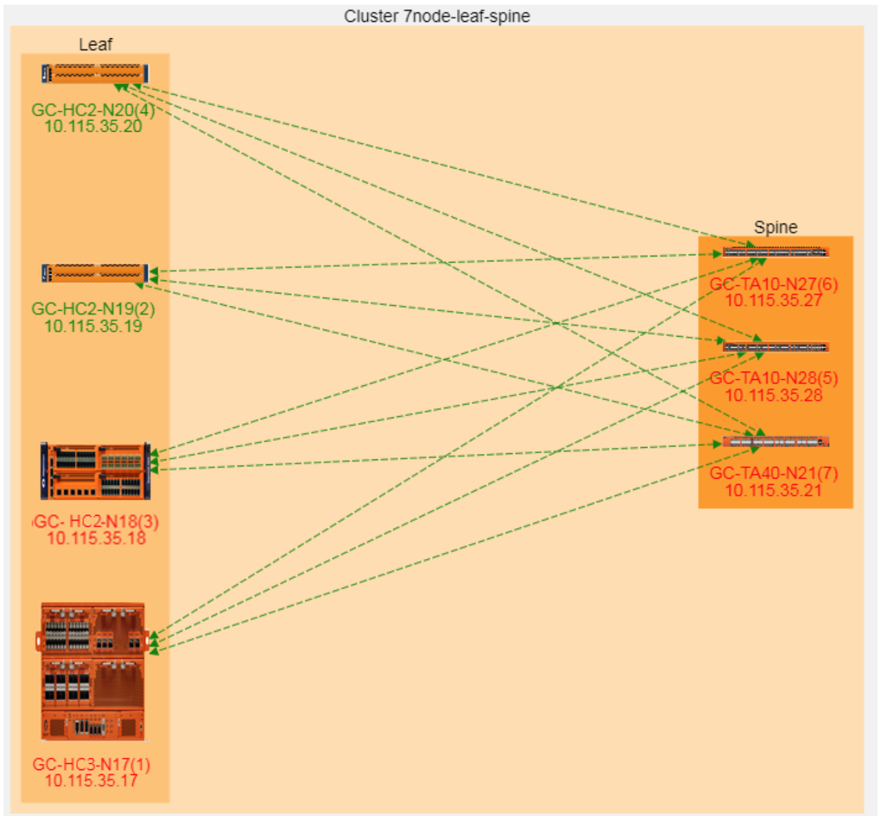
Figure 93 Spine and Leaf Nodes after Selecting Align Cluster Option
