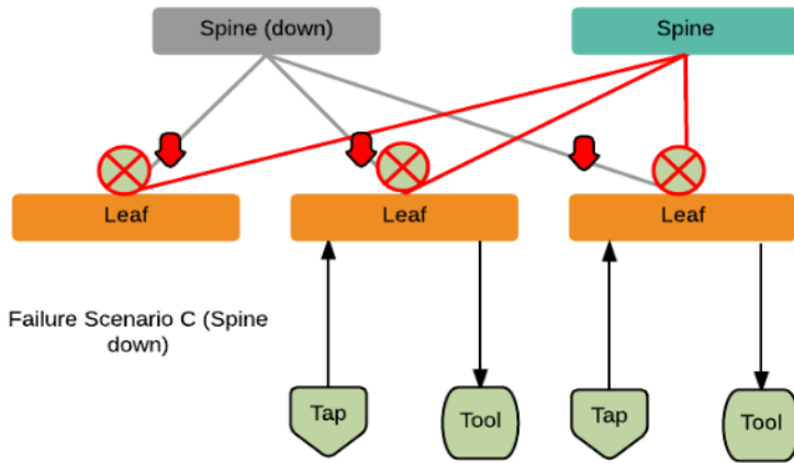
Figure 32 Spine Node Failure
