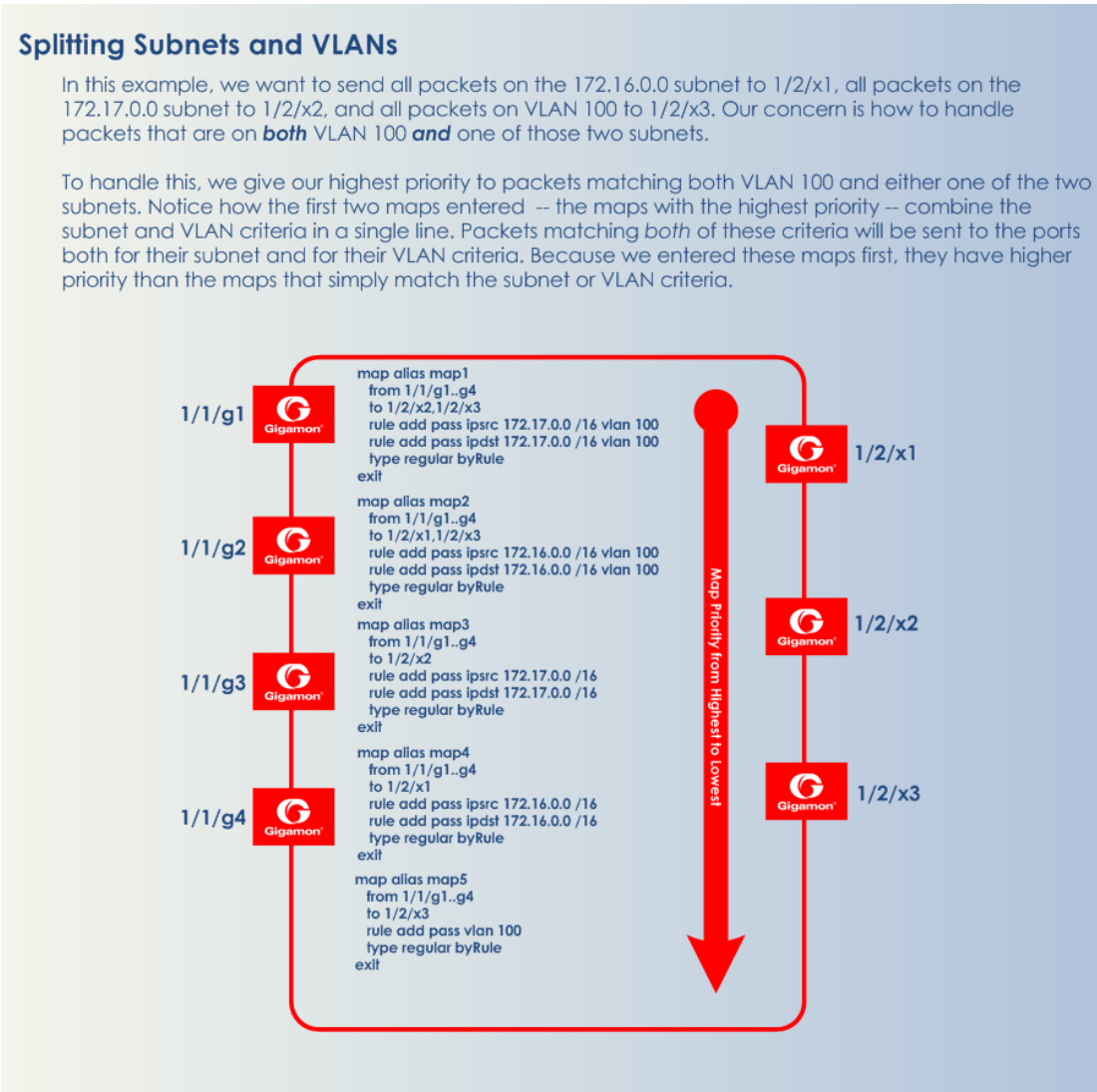
Figure 45 Sending Subnets and VLANs to Different Ports
