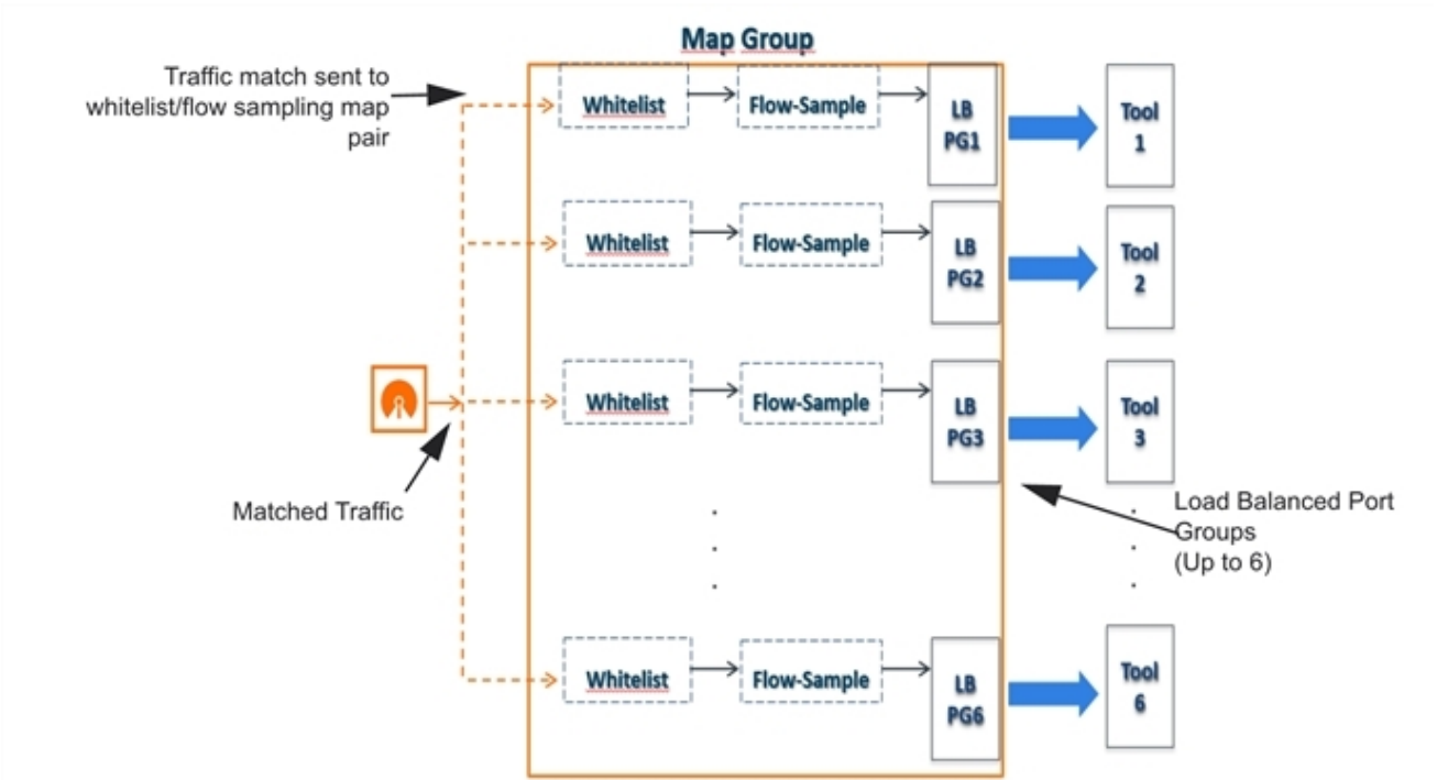
Figure 37 GTP Overlap Flow Sampling Map Groups
