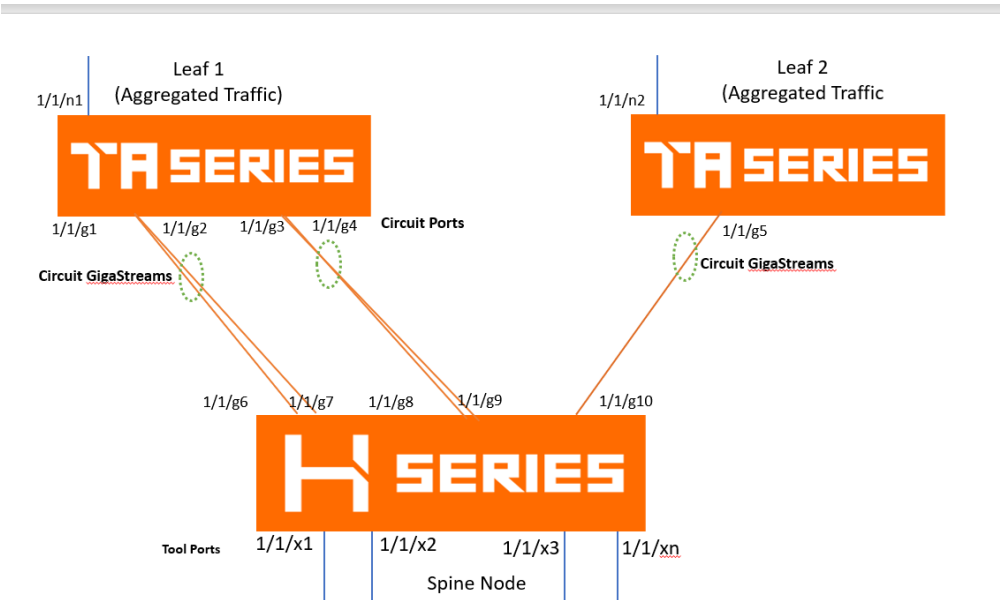
Figure 134 Circuit GigaStreams in Fabric Maps
