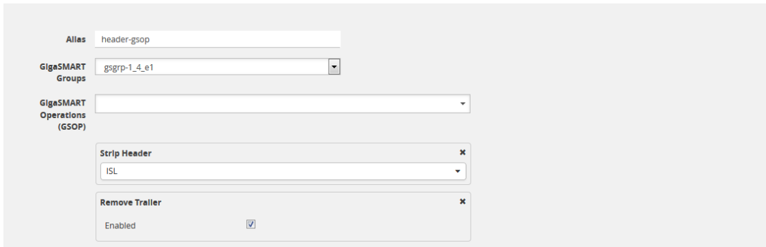
Figure 55 Tunnel Stripping GigaSMART Operation Configured
