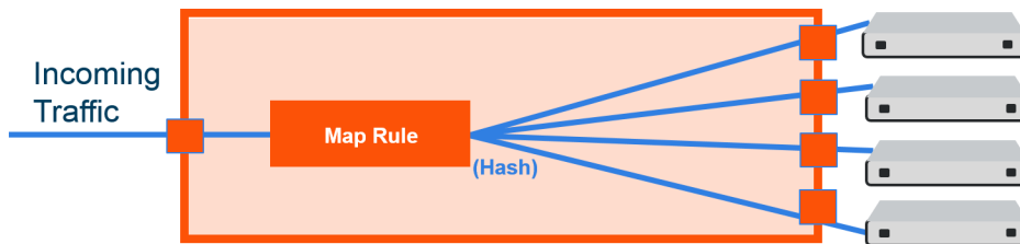
Figure 17 Regular GigaStream Overview
