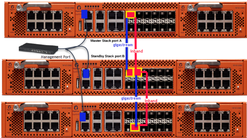
Figure 15 Inband Cluster Management Stack Port Configuration on GigaVUE-HC1
