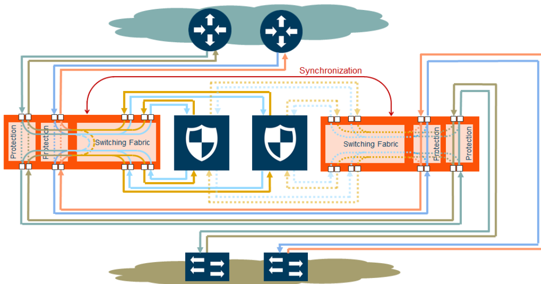
Figure 114 Traffic Flows Through Node with Primary Role
