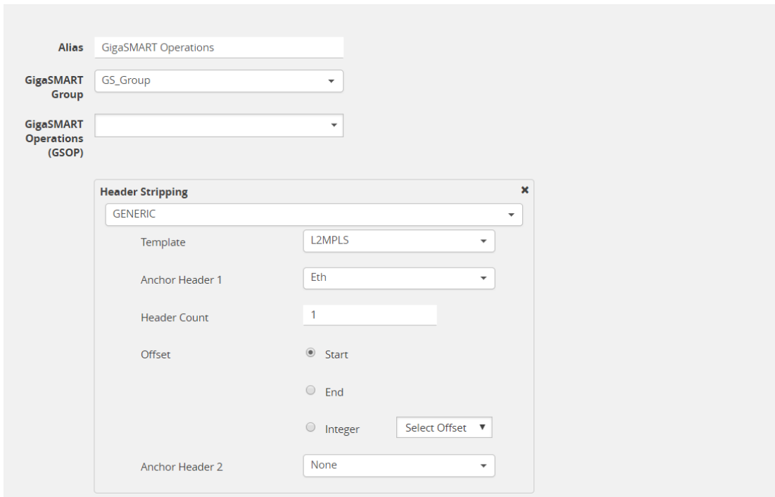
Figure 70 Generic Header Stripping - L2 MPLS
