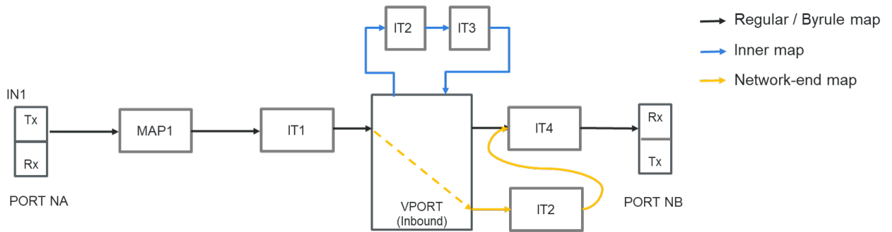
Figure 67 Flexible Inline Decryption Maps
